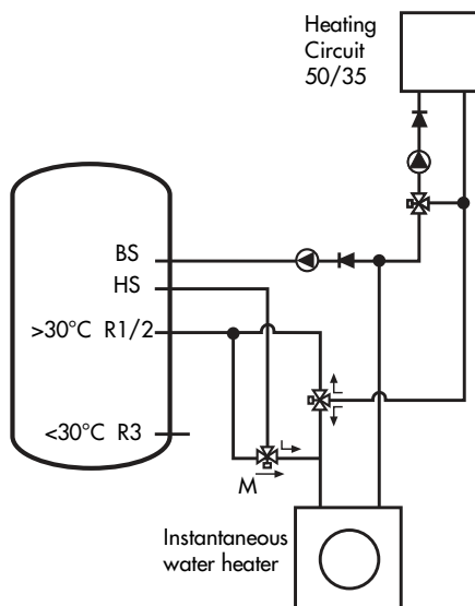
Example 9: Limiting the boiler return temperature
