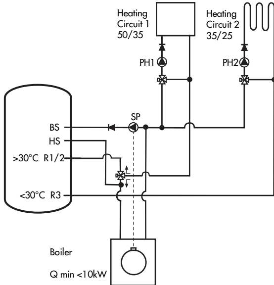
Example 8: Heating circuit 1: 50/35, Heating circuit 2: 35/25
