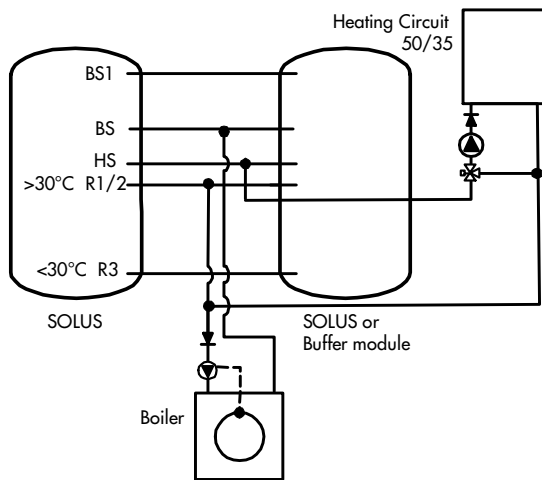
Example 10: Heating circuit 50/35, oil boiler
