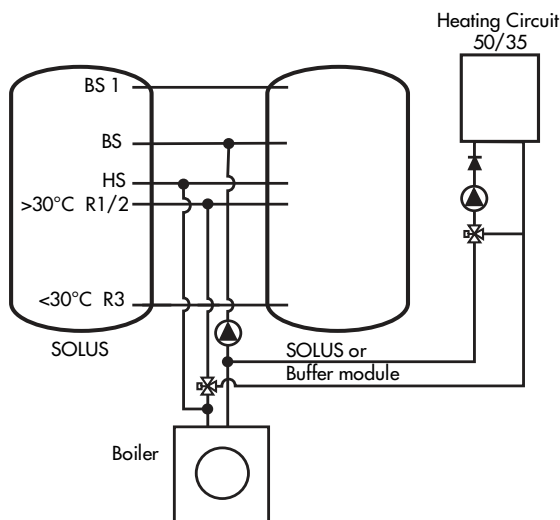
Example 11: Heating circuit 50/35, oil or gas boiler
