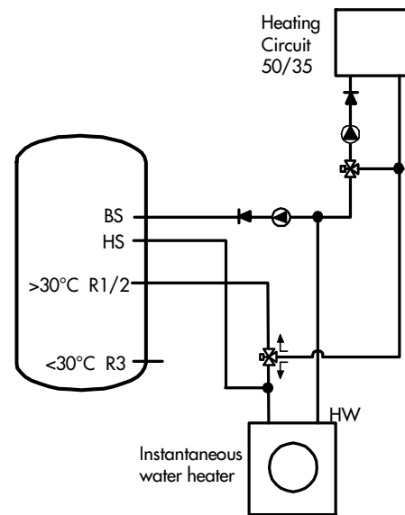
Example 6: Heating circuit 50/35
